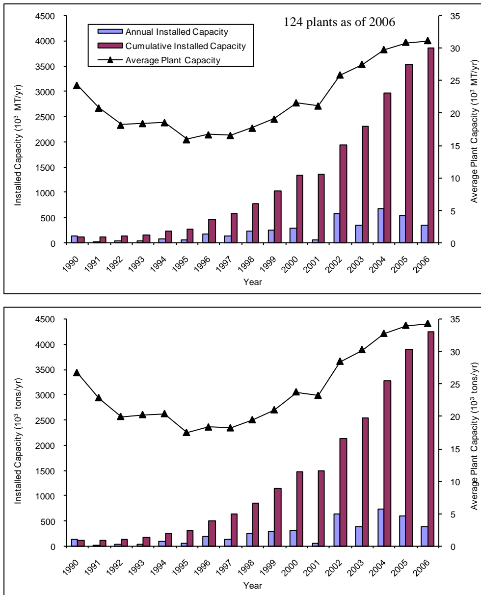
Figure 27. Solid waste anaerobic digester capacity in Europe
