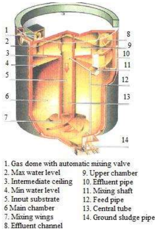
Figure 11. The BIMA digester designed by Entec Biogas GmbH
