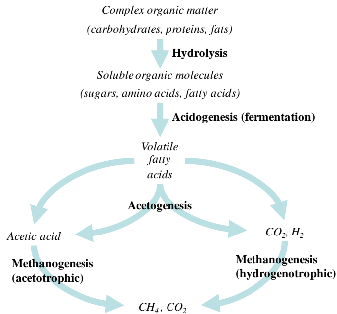
Figure 1. Anaerobic digestion biochemical conversion pathways
