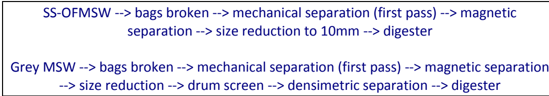
Figure 7. Bassano, Italy pre-processing diagram. Adapted from Bolzonella [41].
