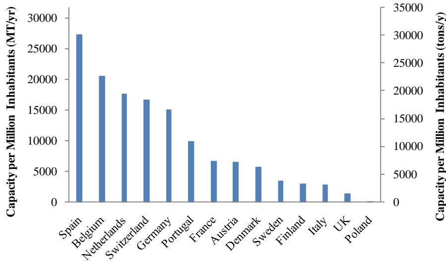
Figure 28. Anaerobic digester capacity by country
