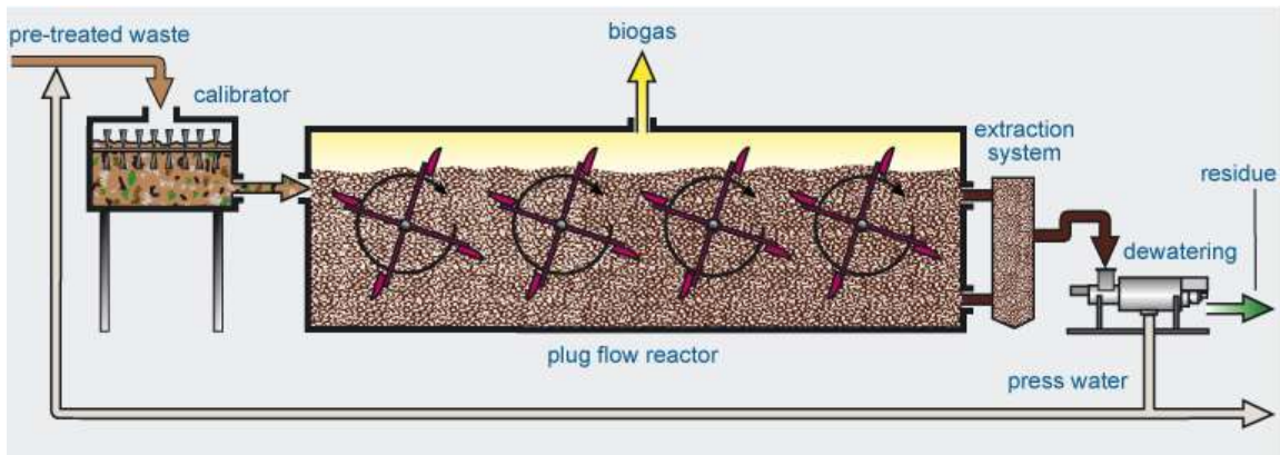
Figure 18. Linde-KCA two-stage dry digester From the Linde-KCA website, accessed September 2007.
