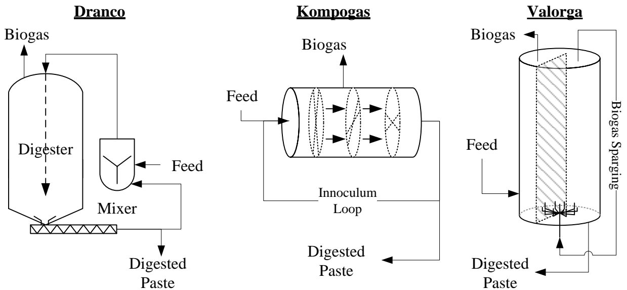
Figure 12. High-solids single-stage digester designs
