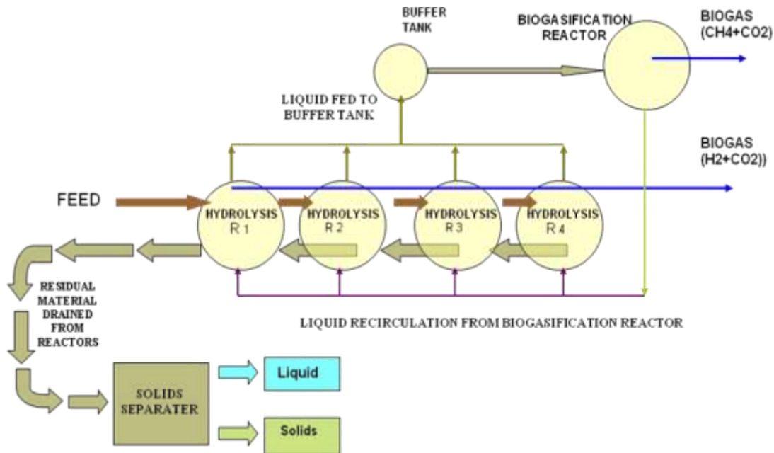
Figure 23. Schematic diagram of the APS Digester system.
