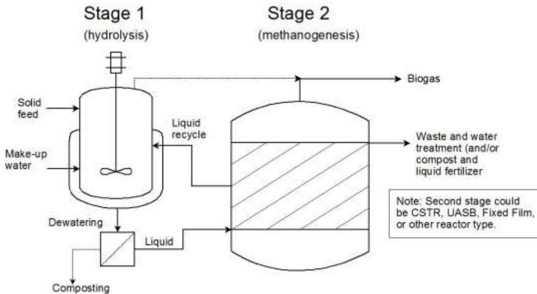
Figure 16. Schematic of a generalized two-stage anaerobic digestion system
