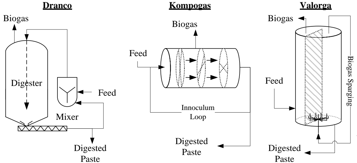
Figure 12). All three systems operate as plug-flow digesters.
