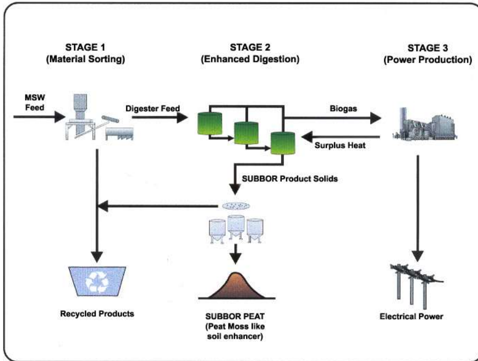
Figure 19. Simplified flow diagram of the two-stage SUBBOR anaerobic digestion process.
