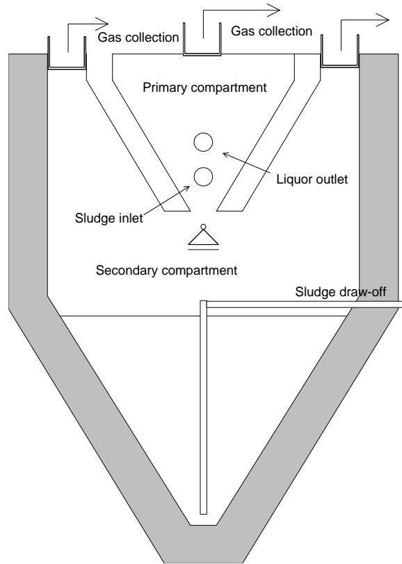
Figure 26. Experimental two-stage garbage digester Developed at the University of Illinois in 1936 [70].
