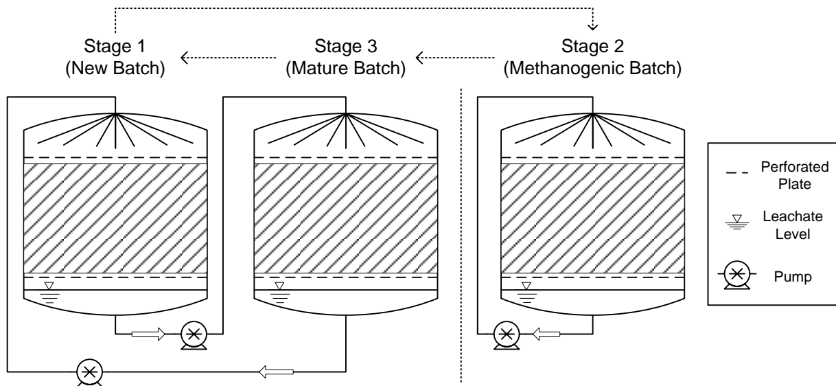
Figure 22. SEBAC process diagram
