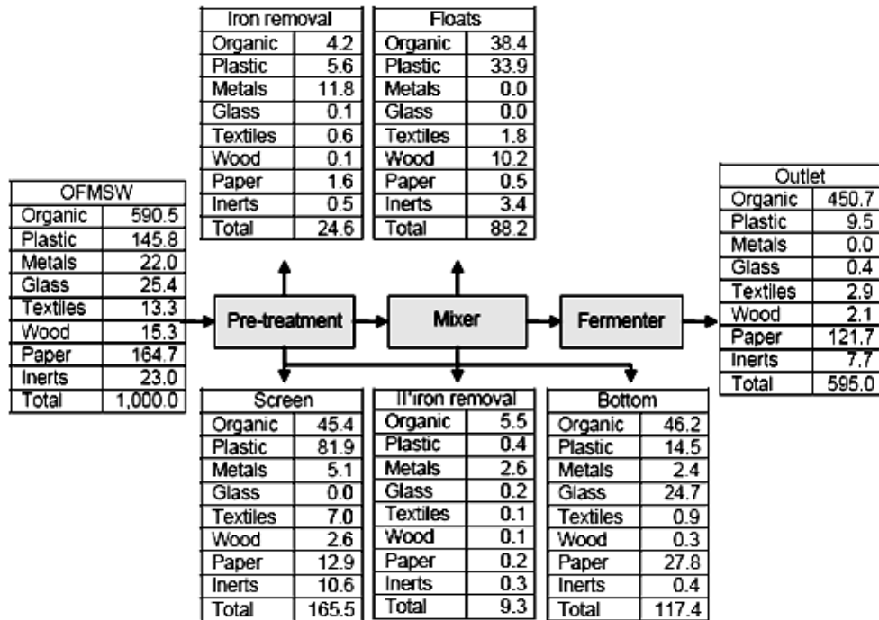
Figure 8. Mass balance of the Treviso wastewater treatment digester sorting line
