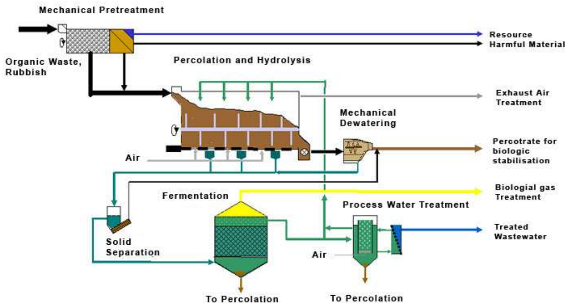
Figure 20. Schematic waste-flow diagram of the two-stage Biopercolat process From the WEHRLE Umwelt GmbH website accessed February 2008.
