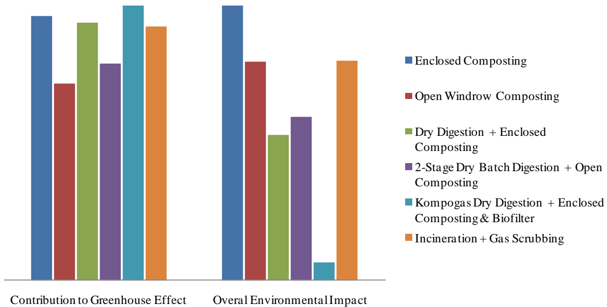
Figure 30. Greenhouse effect contribution and overall environmental impact of 10,000 MT/y (11,000 tons/y) biogenic waste treatment.
