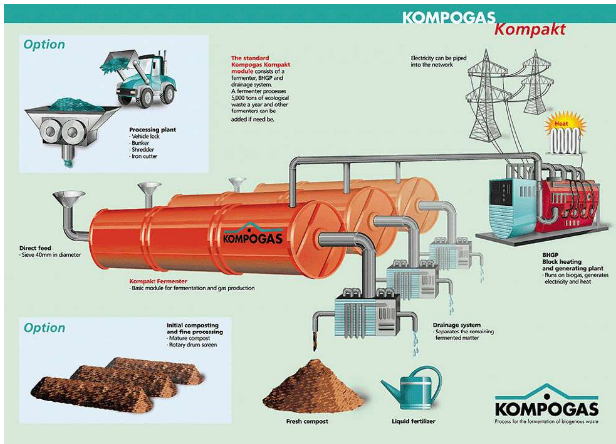
Figure 15. Overview of the KompoGas process From the company website, accessed September 2007.
