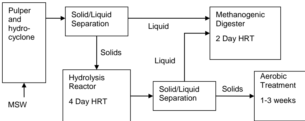
Figure 17. Diagram of the BTA multistage digestion process Adapted from a BTA short information brochure [52].
